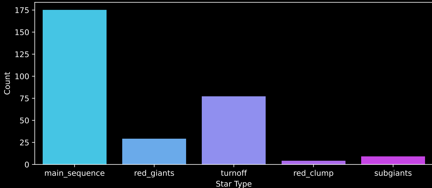
GALAH DR4 Field: [6918] Count plot of Star Type
