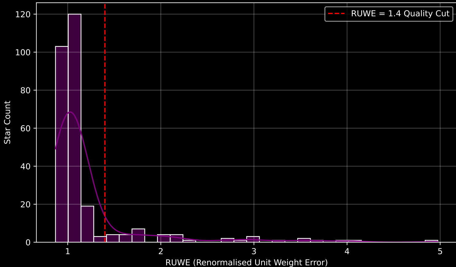
GALAH DR4 Field [6918] RUWE Distribution (n= 282)
